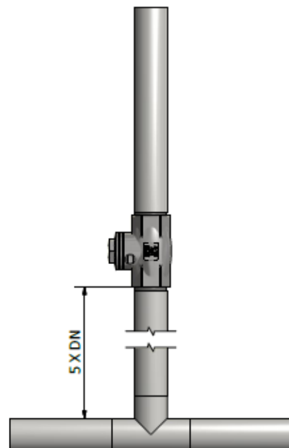
Fig. 3257 vertical Installation after bend
