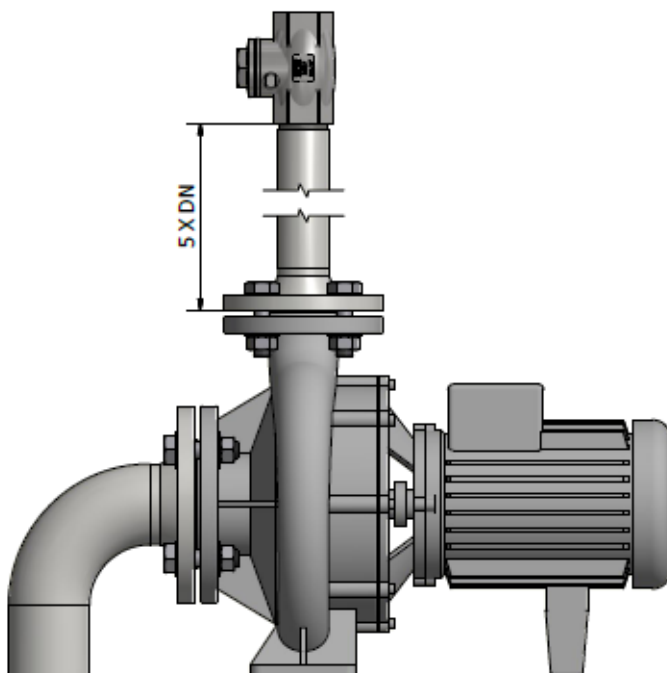
Fig. 3257 vertical Installation after pump
